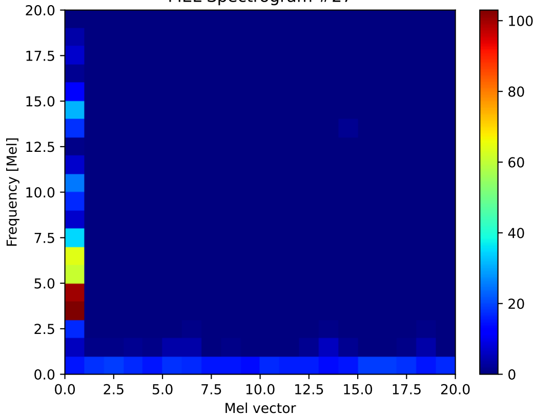
MEL Spectrogram #27
